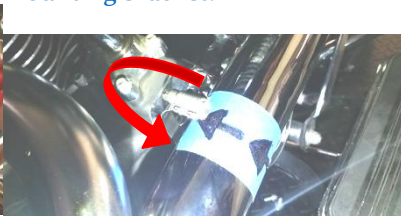
Figure 2.15 Install front shield use a 5/16" nut driver.
