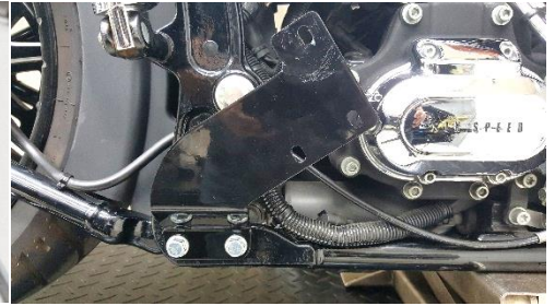
Figure 2.6 install mounting bracket.
