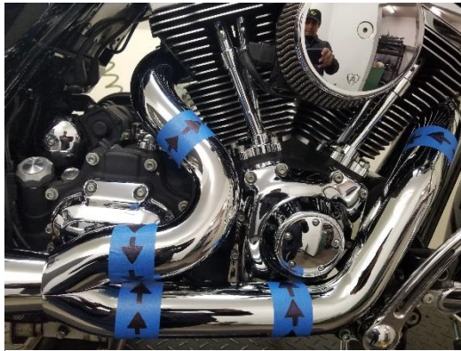
Figure 2.16 Install rear shield.
