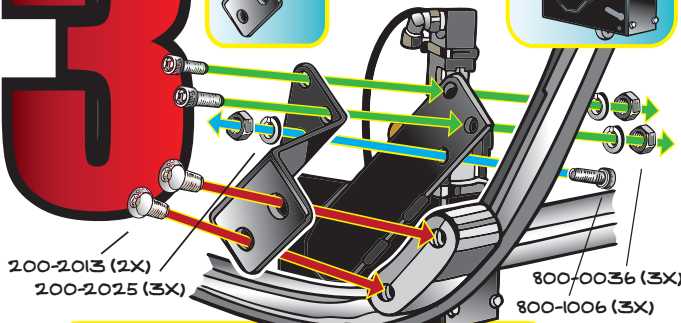
FIGURE C- 2008+ (LEFT SHOCK)
