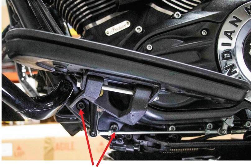
Floorboard Bolts
