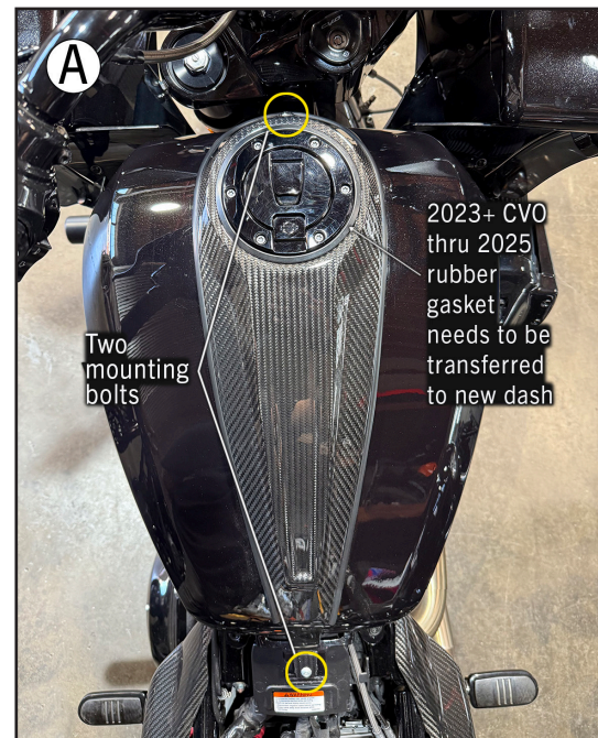
All dash panels install using a bolt at both ends of the dash, top and bottom (yellow circles)
